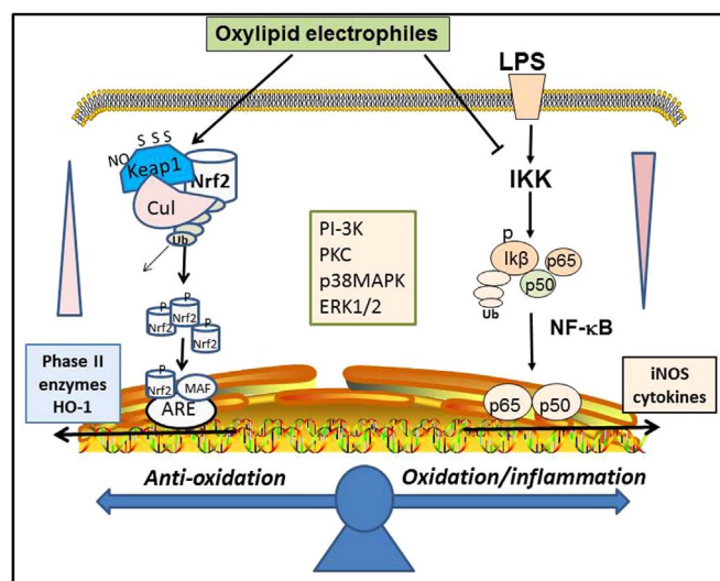
Fig. 3. Oxylipid electrophiles inhibit LPS-induced NF-κB inflammatory pathway and enhance Nrf2/ARE anti-oxidant pathway in microglial cells. Possible cross-talk mediated by protein kinases.
